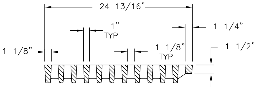
GRATE SECTION
