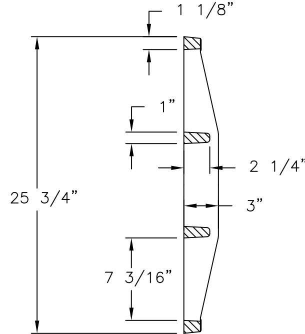
GRATE SECTION
